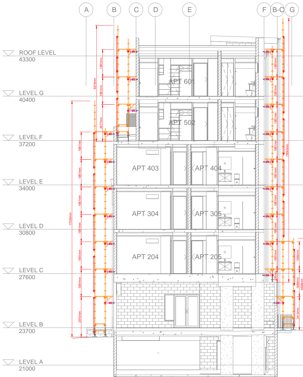
SECTION 01 Scale 1: 100 @ A3
